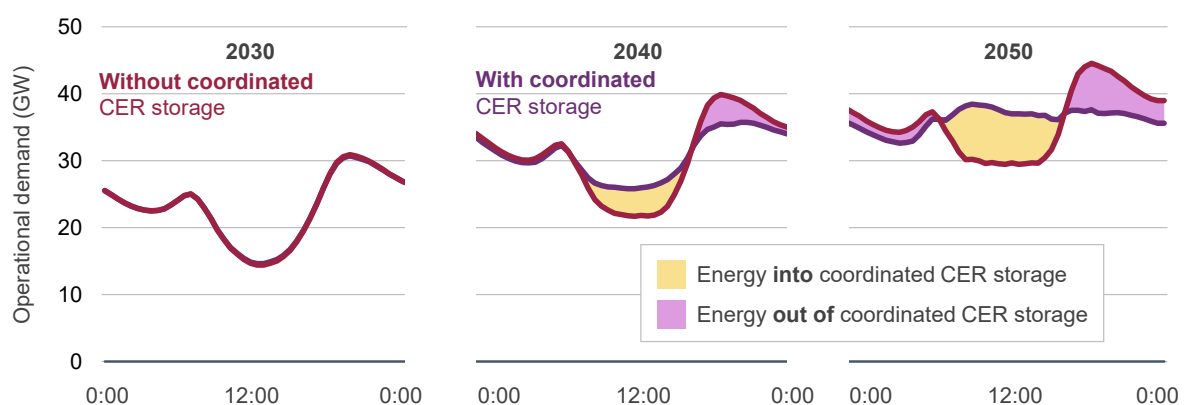
Figure 21 Impact of coordinated CER on average operational demand by time of day, NEM (GW, 2030 to 2050, Step Change)
