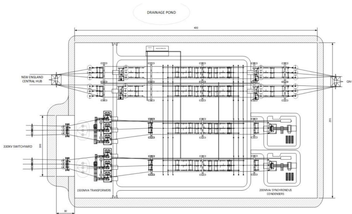
Figure 18: Option 3 Proposed Dumaresq 500/330 kV Substation
