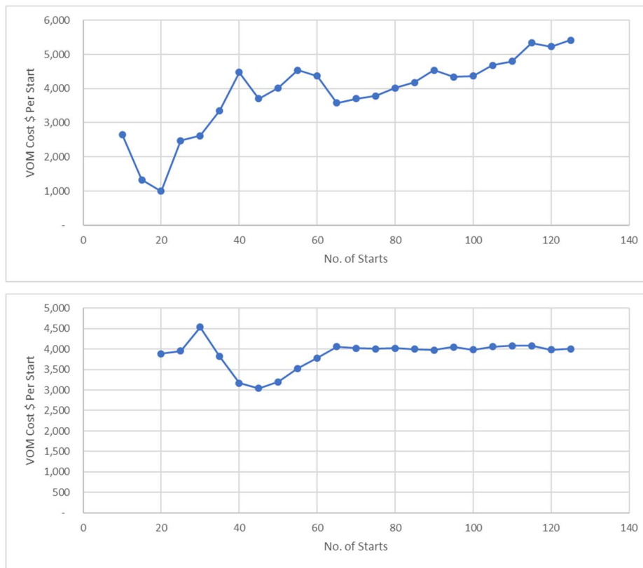
Figure 25: Relationship between Variable O&M Costs per start and number of starts – Parkeston Units (2 and 3 only)
