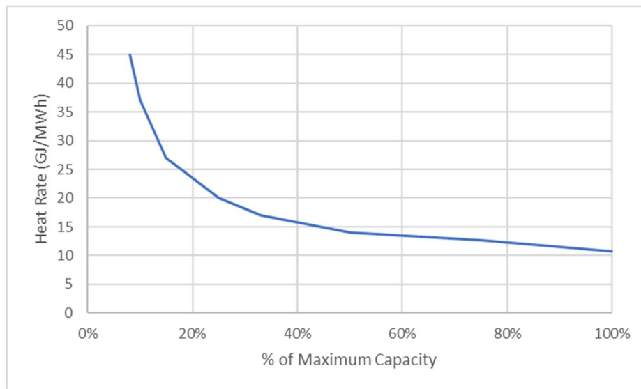
Figure 14: Typical heat rate 40 MW Aero Derivative Units
