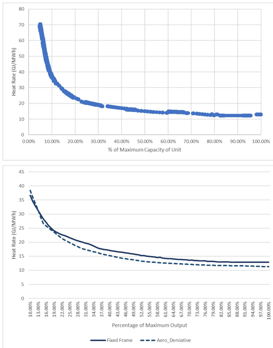
Figure 12: Typical Heat Rate of 40 MW OCGT Units — 15 Degrees Celsius / 30 percent humidity — Fixed Frame and Aero-Derivative Units
