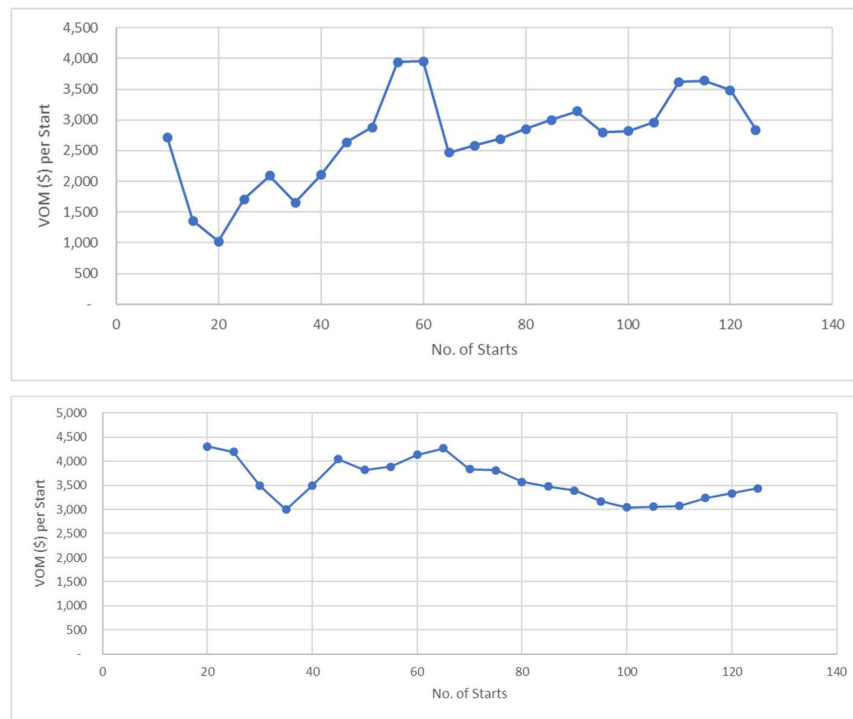
Figure 6: Relationship between Variable O&M Costs per start and number of starts – Pinjar Units
